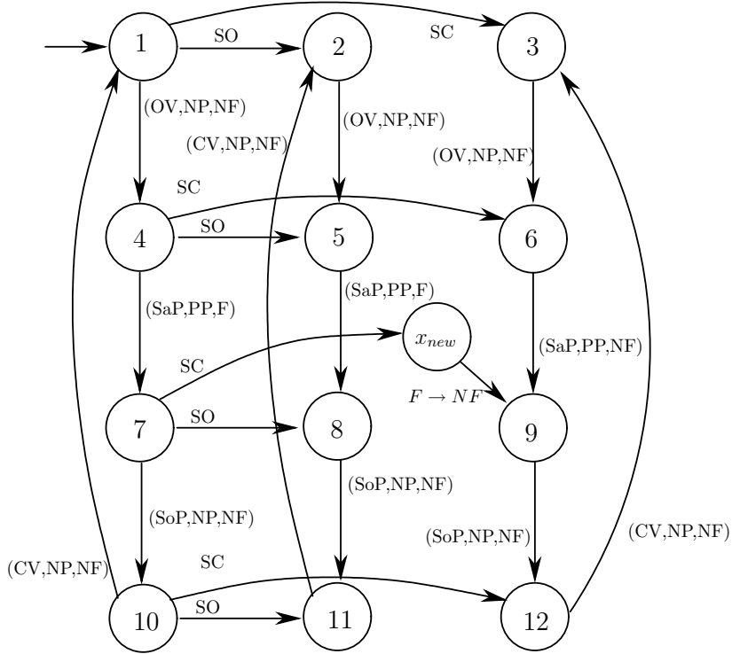
Figure 2.32: Complete model of pump, valve, and controller, together with flow sensor and pressure sensor (Example 2.25).
