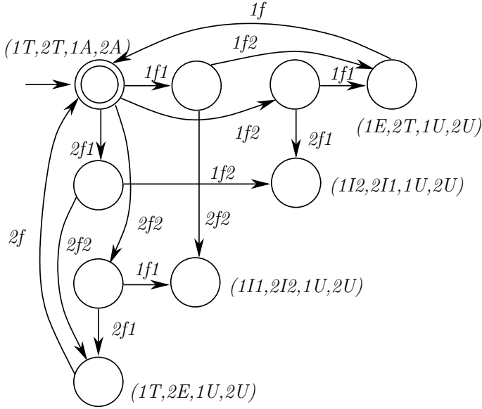
Figure 2.19: The parallel composition of the four automata in Fig. 2.18 (Example 2.18).
