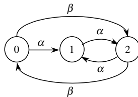
Figure 6.1: State transition diagram for Example 6.2.
