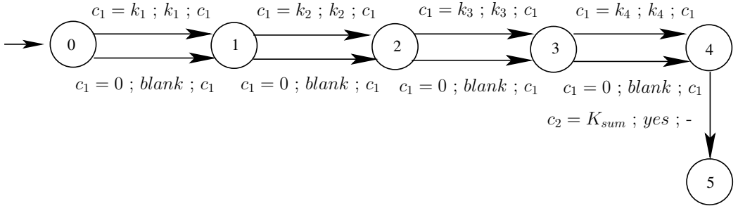
Figure 5.19: Timed automaton with guards G_{tg}^{sum} of Example 5.6 that encodes the subset sum problem for a given set of four integers K = \{k_1, k_2, k_3, k_4\} and a desired sum K_{sum} . State 5 will only be reached if there is a subset of K whose elements sum up to K_{sum} .
