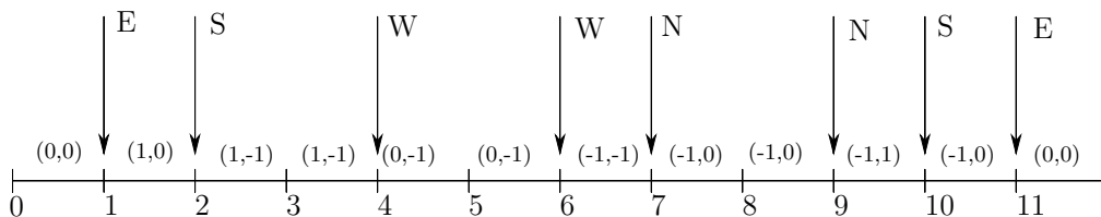
Figure 1.21: Event-driven random walk on a plane.
