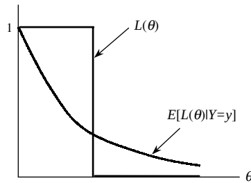
Figure 11.30: Illustrating the smoothing property of the conditional expectation.
