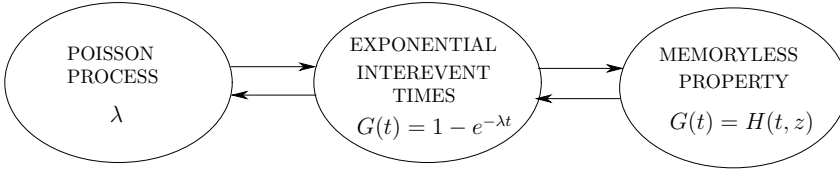
Figure 6.10: Properties of the Poisson process.
