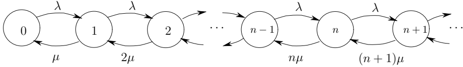
Figure 8.10: State transition rate diagram for the M/M/\infty system.
