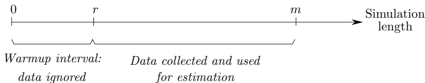
Figure 10.12: Illustrating the initial data deletion approach for non-terminating simulations.
