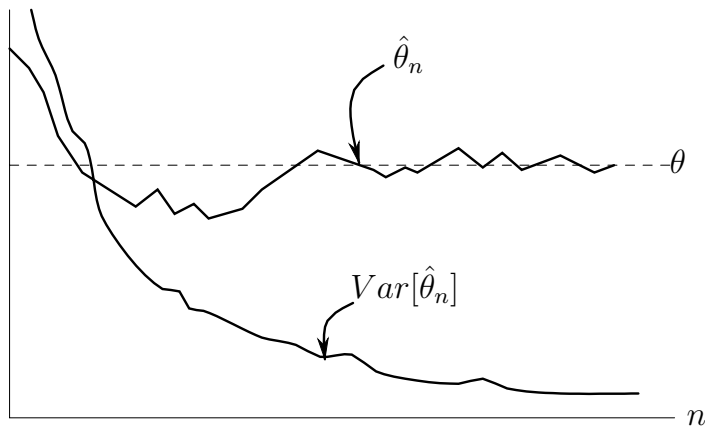
Figure 10.10: Typical behavior of a strongly consistent point estimator \hat{\theta}_n and its variance \text{Var}[\hat{\theta}_n] as a function of the number of data n .
