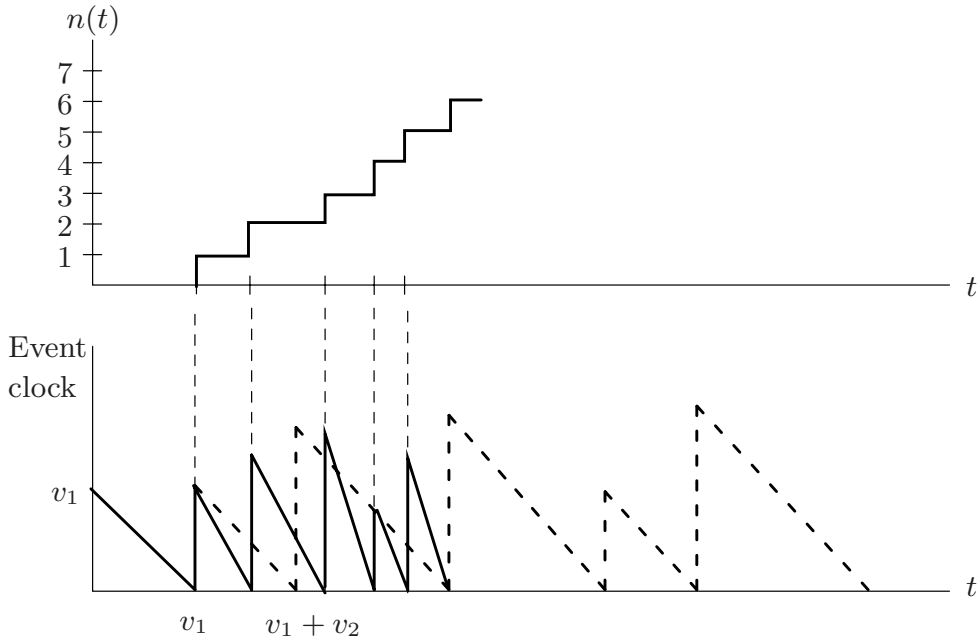
Figure 6.14: A counting process with a variable-speed event clock.
