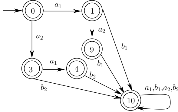
Figure 3.6: Reduced-state realization of supervisor in Examples 3.7 and 3.6.
