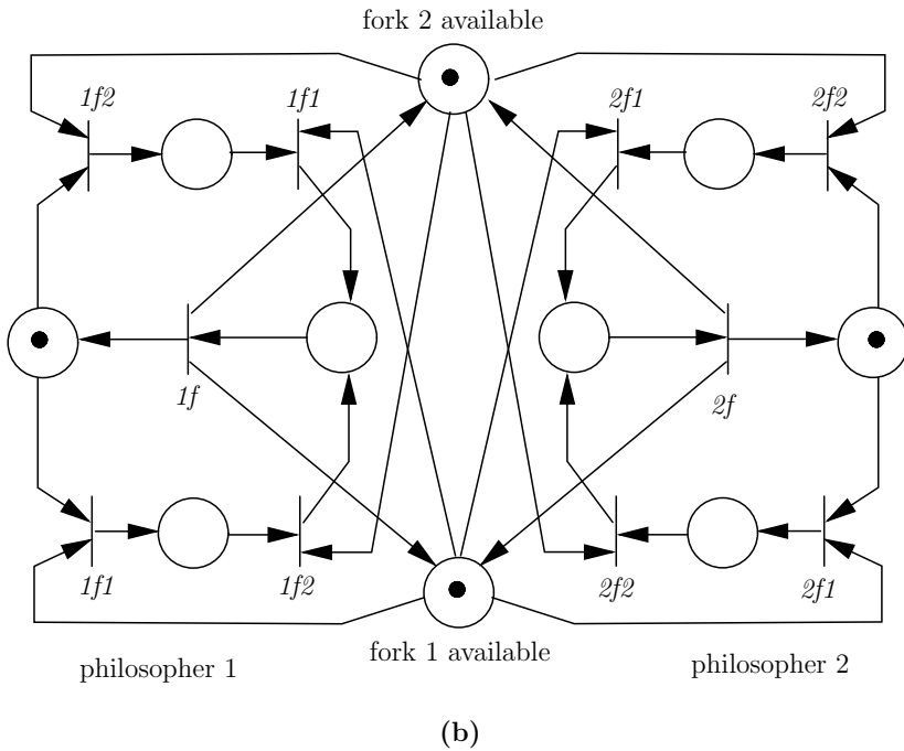
Figure 4.9: Petri net model of the dining philosophers example, with two philosophers and two forks. (Example 4.6).
