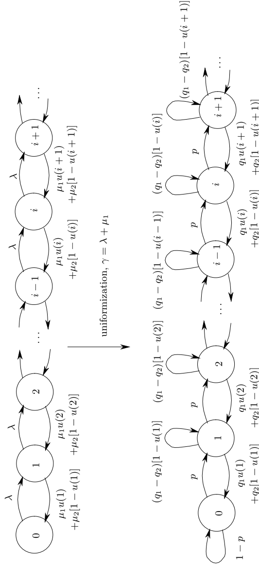
Figure 9.2: Markov chain model and its uniformization for Example 9.2.
