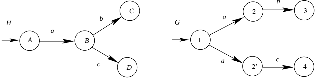
Figure 2.23: Equivalence of automata.
