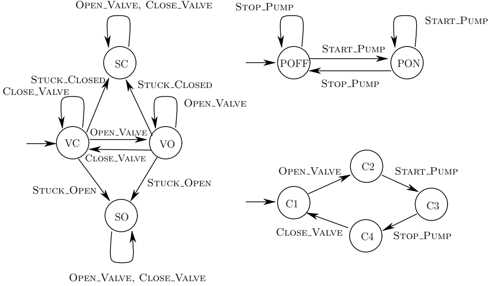
Figure 2.31: Component models of pump, valve, and controller (Example 2.25).
