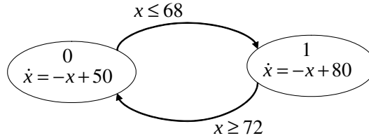
Figure 5.27: A simple thermostat as a hybrid system.
