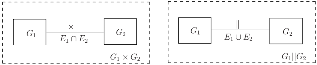
Figure 2.14: This figure illustrates the interconnection of two automata.
