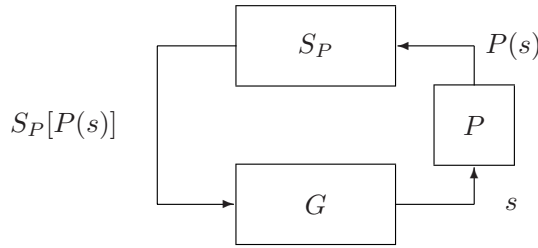
Figure 3.2: The feedback loop of supervisory control in the case of partial observation. The projection P : E^* \rightarrow E_o^* hides the unobservable events executed by G from supervisor S_P .
