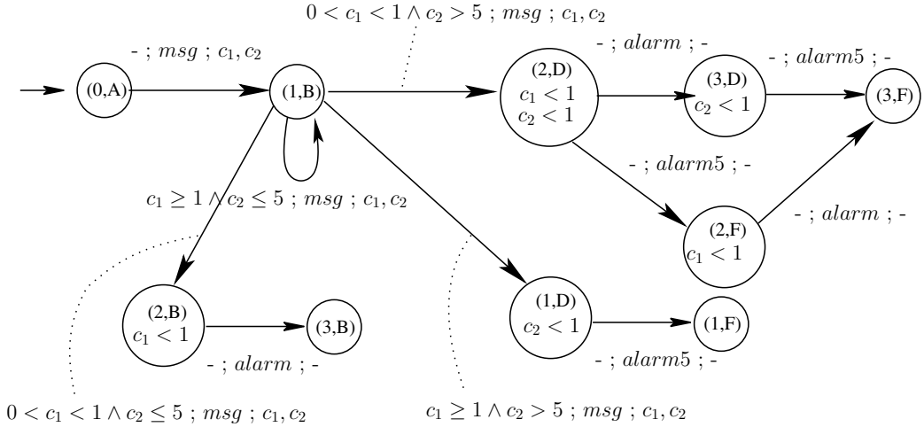
Figure 5.21: Parallel composition of G_{tg}^{ai} of Fig. 5.18 and G_{tg}^{ai5} of Fig. 5.20 (Example 5.7). It can be inferred that state (2, D) is never reached.
