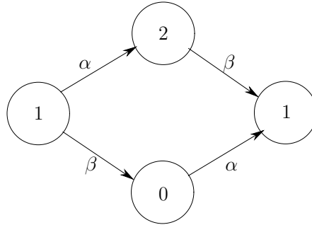
Figure 11.8: The “commuting condition” for the system of Fig. 11.6.
