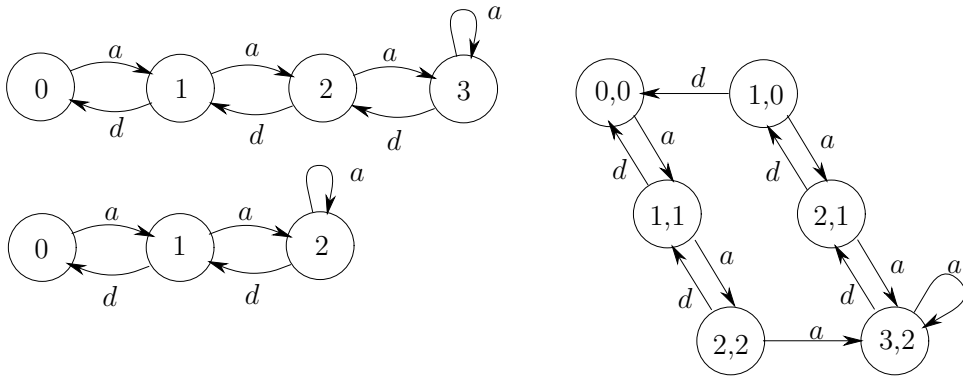
Figure 11.41: State transition diagrams for Example 11.14.
