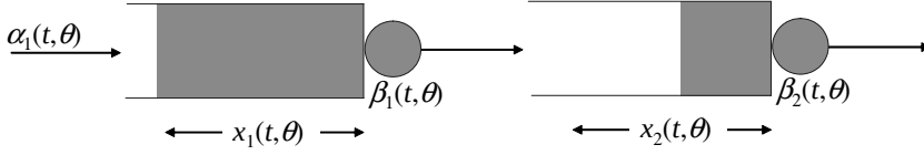
Figure 11.35: A two-node SFM.
