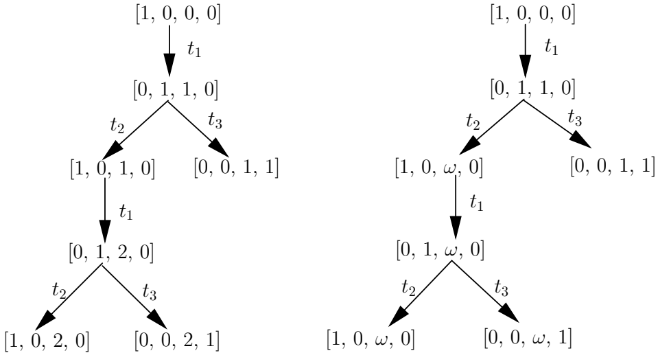
Figure 4.13: Coverability tree construction for Example 4.10.
