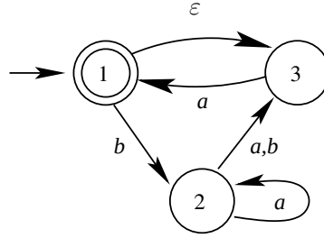
Figure 2.9: Nondeterministic automaton with \varepsilon -transition of Example 2.13.
