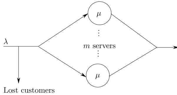
Figure 8.13: The M/M/m/m queueing system.
