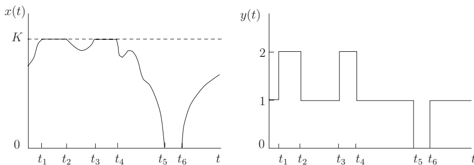
Figure 1.14: Sample paths for Example 1.9.
