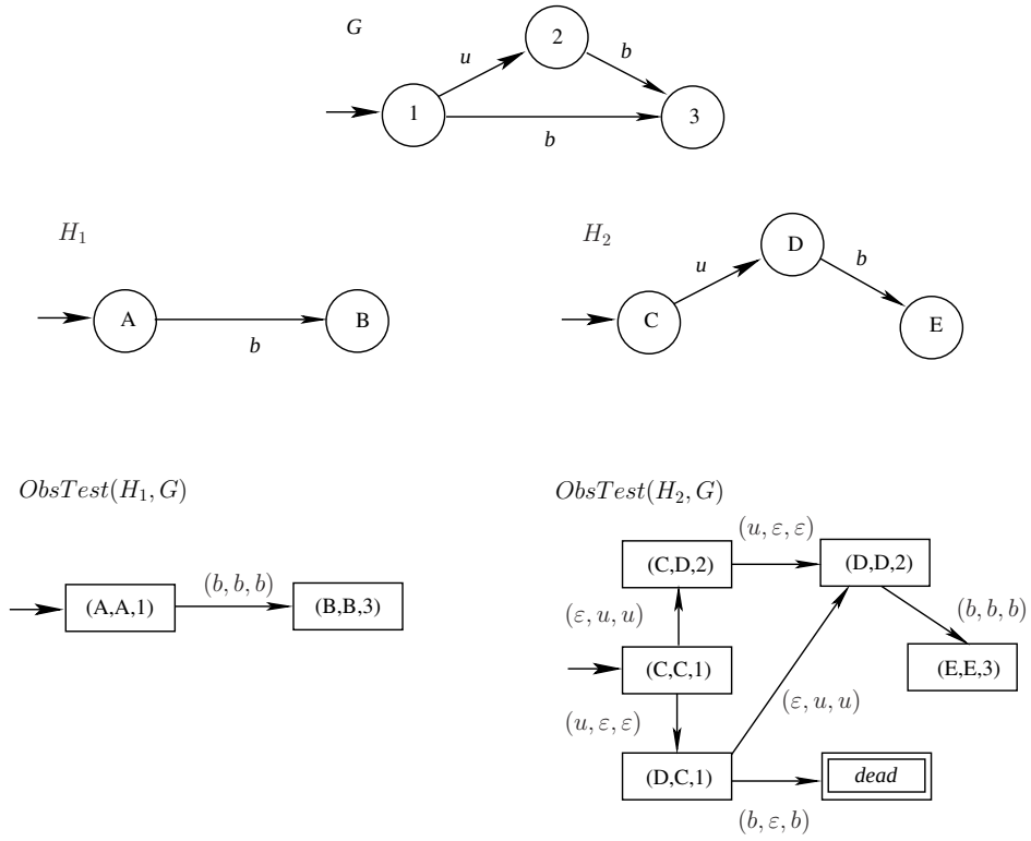
Figure 3.18: ObsTest(H, G) .
