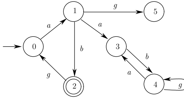
Figure 2.4: Blocking automaton of Example 2.7. State 5 is a deadlock state, and states 3 and 4 are involved in a livelock.
