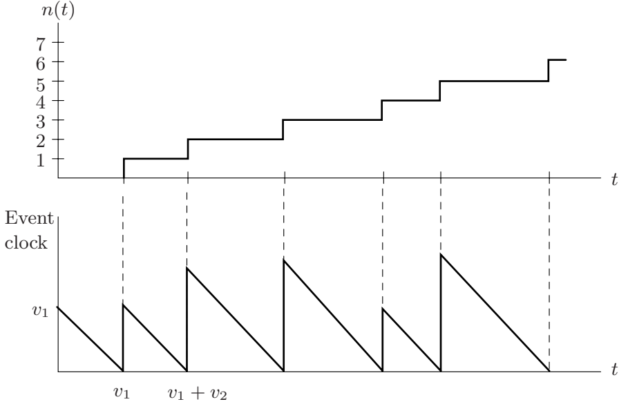
Figure 6.13: A counting process with a fixed-speed event clock.
