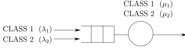
Figure 6.12: Queueing system for Example 6.4.
