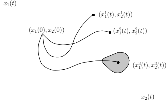
Figure 1.10: Sample paths in a two-dimensional case.
