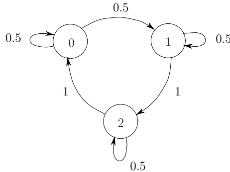
Figure 7.12: Aperiodic states.
