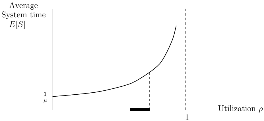
Figure 8.7: Average System Time as a function of utilization in the M/M/1 system.
