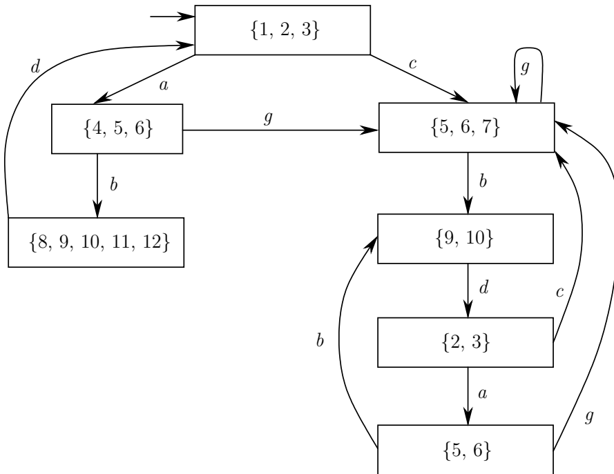
Figure 2.28: Observer G_{obs} of G in Fig. 2.27 (Example 2.24).
